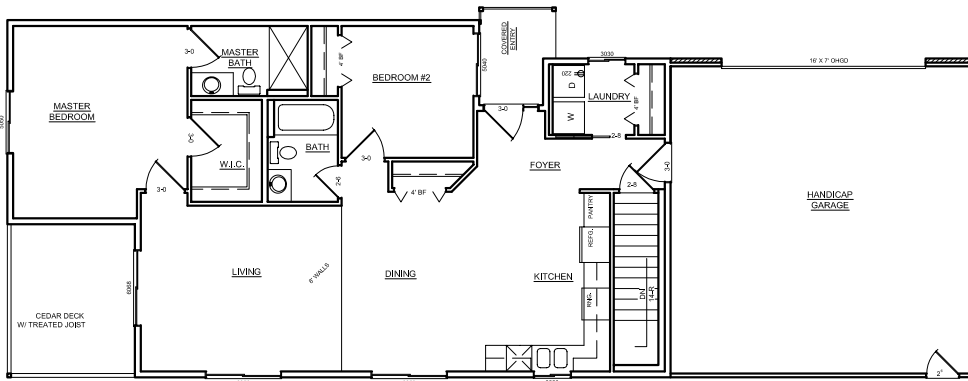
MAIN LEVEL FLOOR PLAN
